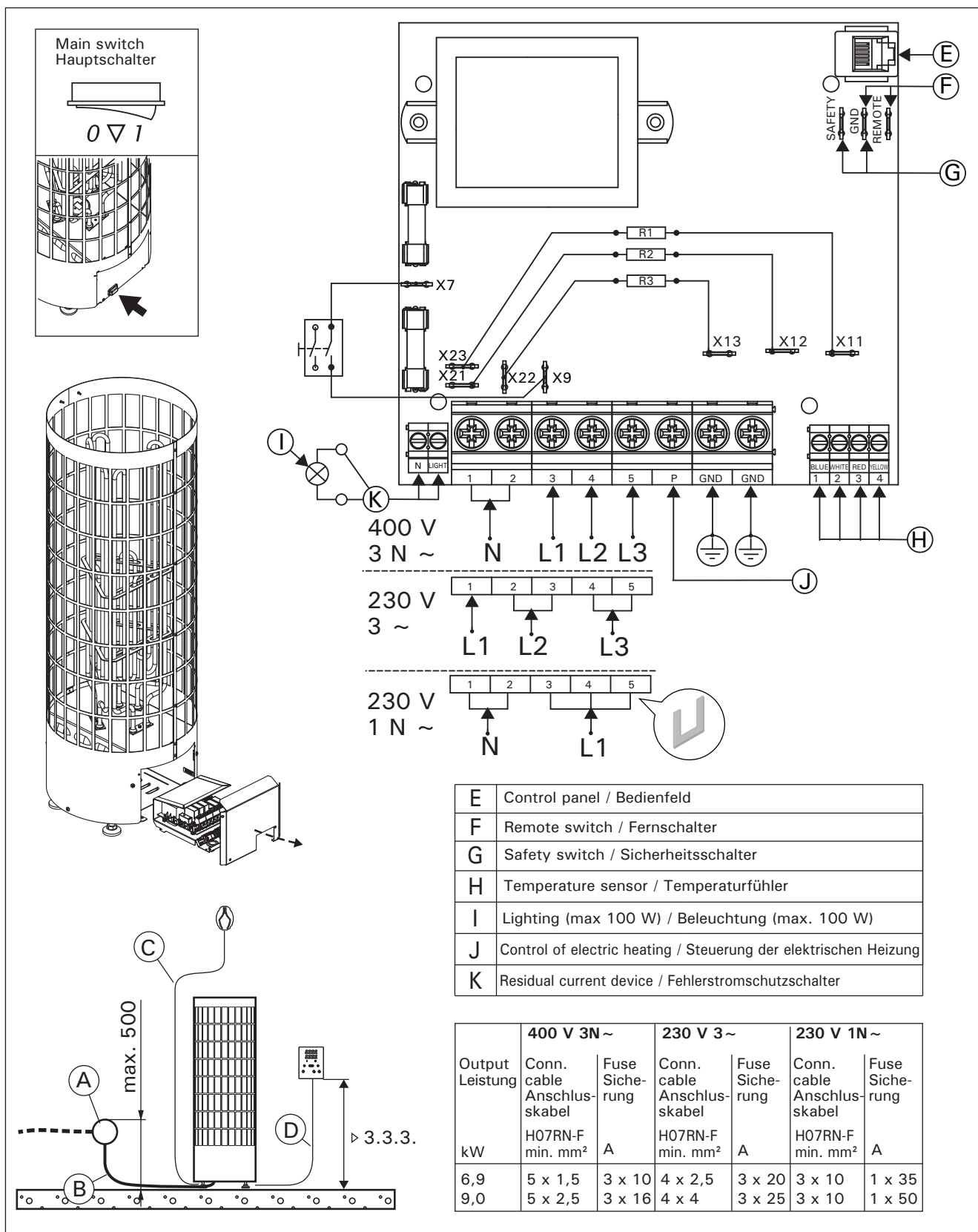
Electrical connections
